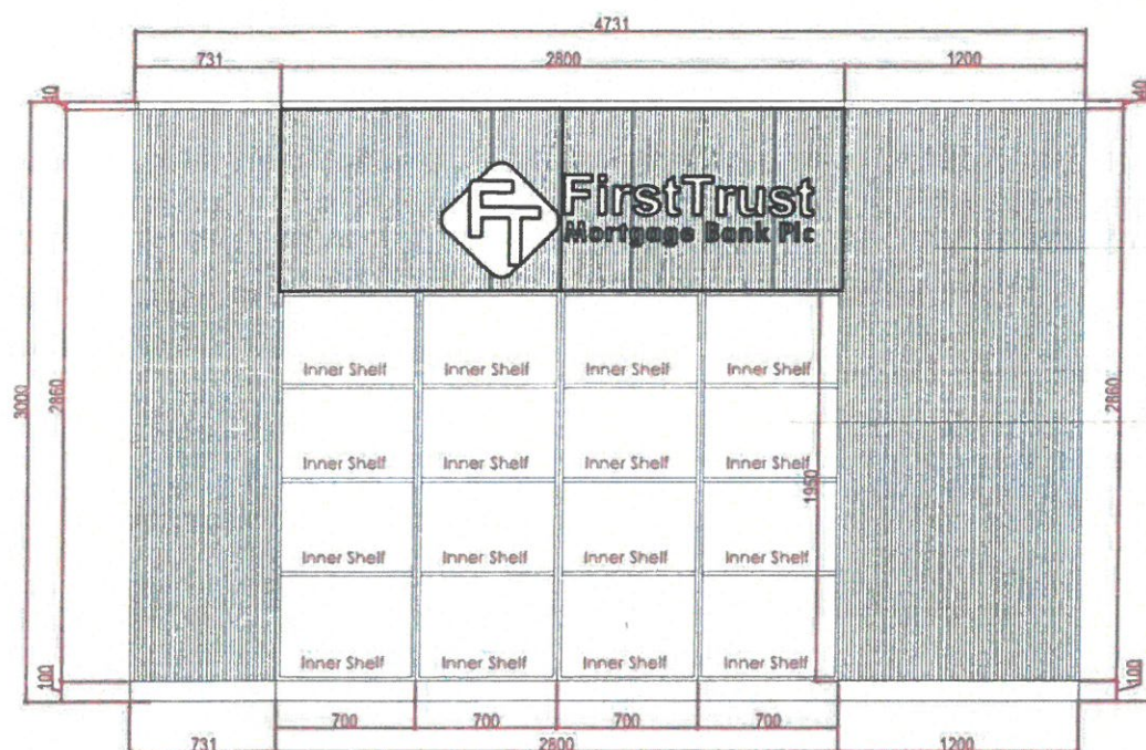
Elevation -C
