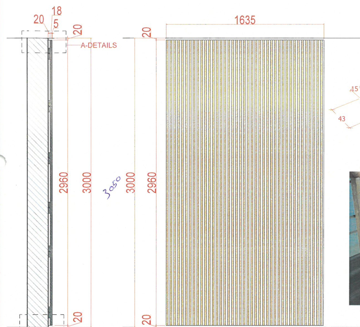
Side view Details
