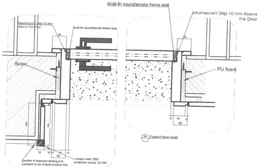
D2 Typical Frame detail
