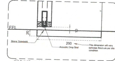
D3 Typical Drop seal detail
