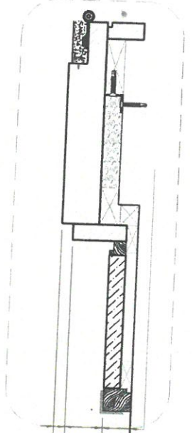
Type A and A mir. architrave
