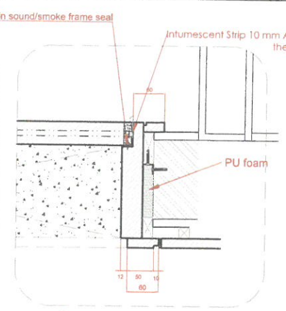
D1 Typical Frame detail
